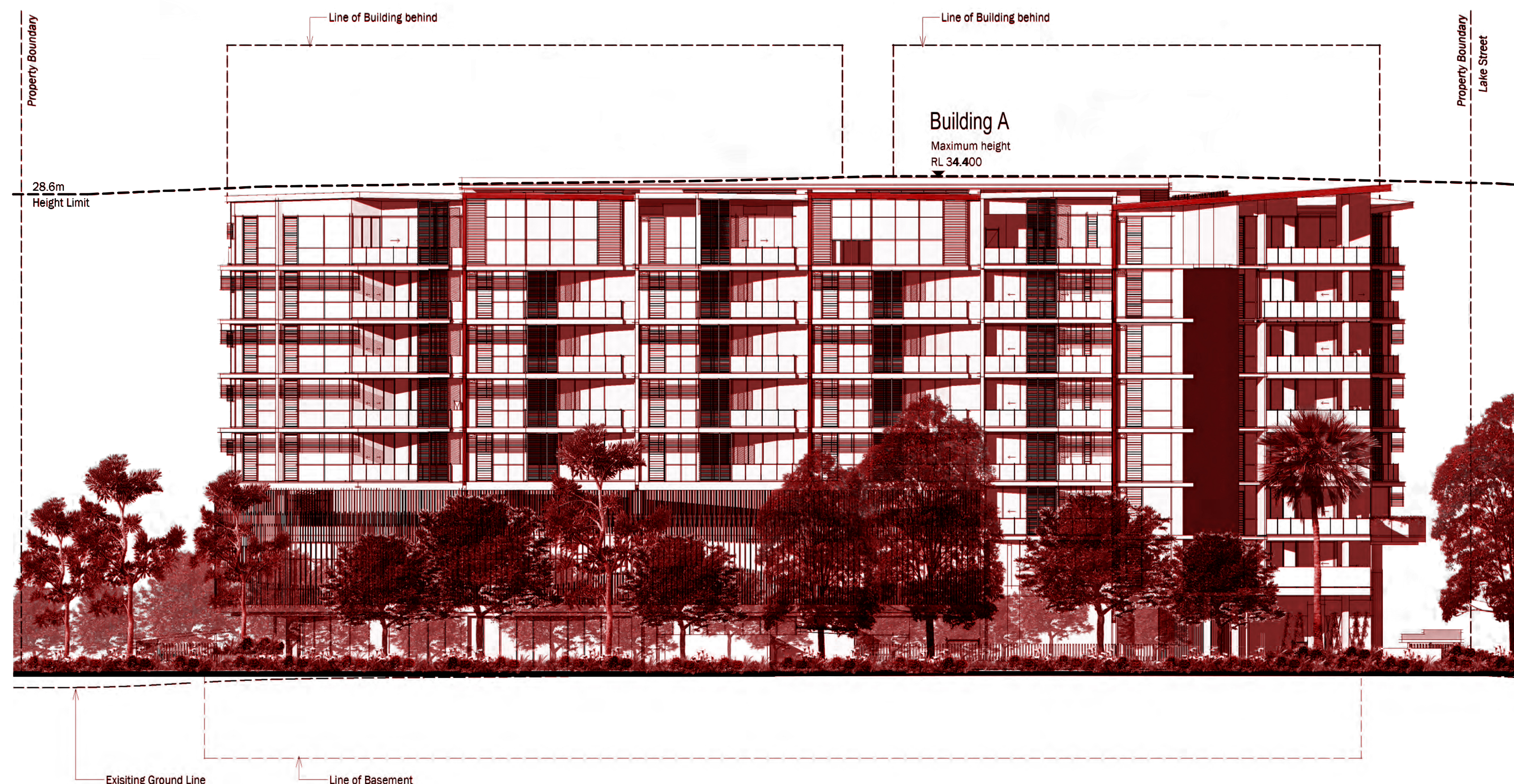
East Elevation
